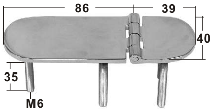
HINGE WITH THREAD precesion casted AISI 316 ITEM NO. WxL mm Thickness mm Weight/g 008621 40x125(1-9/16"x5") 4 182
