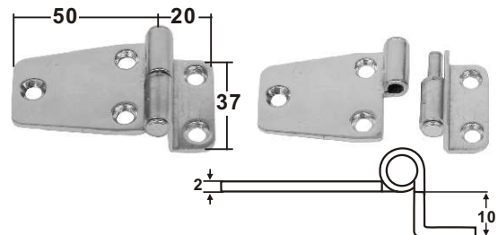
TAKE APART HINGE stamped AISI 304 Thickness:2mm ITEM NO. Weight/g 007001 Right(no picture) 54 007002 Left 54 on request AISI 316
