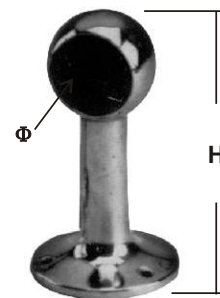
END STANCHIONS casted AISI 316 closed ITEM NO. Φ mm H mm Weight 009893 22 87 206 009764 25 87 188 009765 40 105 306
