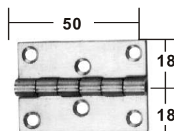
STAMPED AISI 304 buff polished ITEM NO. Thickness Weight/g 006006 1.5 mm 30 on request AISI 316
