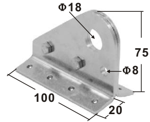
SHROUD PLATE stamped AISI 316 Thickness:3mm ITEM NO. Weight/g 004309 304
