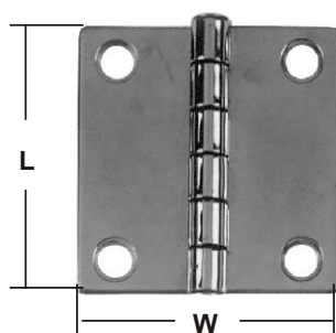
BUTT HINGE stamped AISI 304 thickness:1.5mm ITEM NO. L mm W mm Weight/g 006024 50(2") 50(2") 37 006038 50(2") 38(1-1/2") 31 006075 75(3") 75(3") 81 006039 38(1-1/2") 38(1-1/2") 23 on request AISI 316
