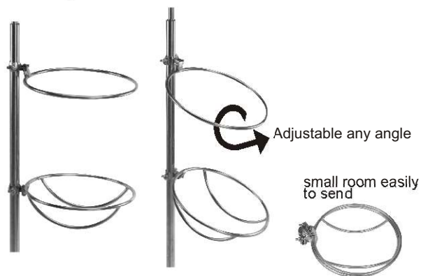
FENDER HOLDER MOVEABLE AISI 316 ITEM NO. fender 007926 \Phi 135mm for 125mm(5") fender 007927 \Phi 160mm for 150mm(6") fender 007929 \Phi 230mm for 200mm(8") fender 007930 \Phi 265mm for 250mm(10") fender
