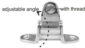
UNIVERSAL DECK HINGE casted AISI 316 ITEM NO. Base Weight/g 009712 3-1/4"x1"(82x25mm) 135
