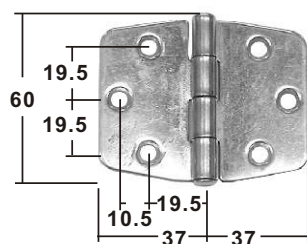
HINGE stamped AISI 304 buff polished ITEM NO. Thickness Weight/g 006009 2 mm 84 on request AISI 316
