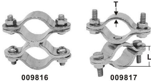
CLAMP stamped AISI 304 ITEM NO. L mm T mm Type Weight/g 009816 19~30 3 fixed 144 009817 19~30 3 swivel 148
