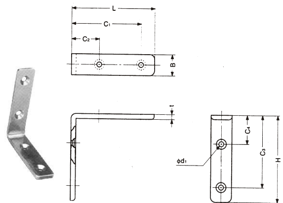
ANGLES stamped AISI 304
