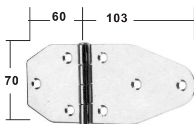
STAMPED AISI 304 buff polished ITEM NO. Thickness Weight/g 006080 2 mm 170 on request AISI 316
