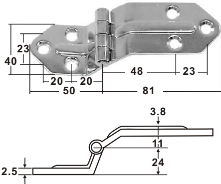
STAMPED AISI 304 buff polished ITEM NO. Thickness Weight/g 006069 2.5 mm 119 on request AISI 316
