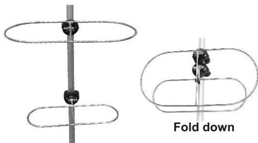
FENDER HOLDER AISI 316 ITEM NO. fender 007933 \Phi 160mm for 150mm(6") double fenders 007934 \Phi 220mm for 210mm(8") double fenders
