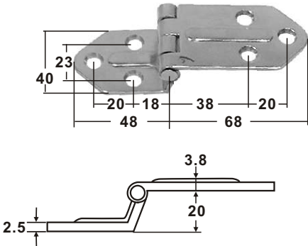
STAMPED AISI 304 buff polished ITEM NO. Thickness Weight/g 006068 2.5 mm 98 on request AISI 316
