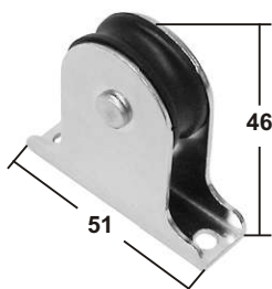
SINGLE LEAD BLOCK AISI 304 For rope \Phi 6 mm plastic sheaves 30x11mm ITEM NO. Weight 012011 46g
