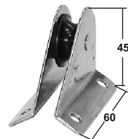
SINGLE LEAD BLOCK AISI 304 For rope \Phi 4 \sim \Phi 6 mm plastic sheaves 25x9.2mm ITEM NO. Weight 012025
