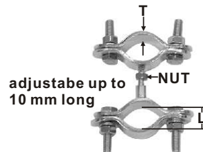
SWIVEL CLAMP stamped AISI 304 can adjust ITEM NO. L mm T mm Weight/g 009807 19~25 3 154
