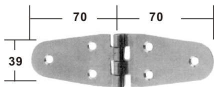
STAMPED AISI 304 buff polished ITEM NO. Thickness Type Weight/g 006014 2 mm 81 006054 2 mm reverse 81 on request AISI 316
