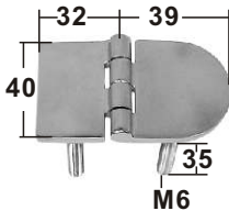
HINGE WITH THREAD precesion casted AISI 316 ITEM NO. WxL mm Thickness mm Weight/g 008623 40x69(1-9/16"x2-3/4") 4 114
