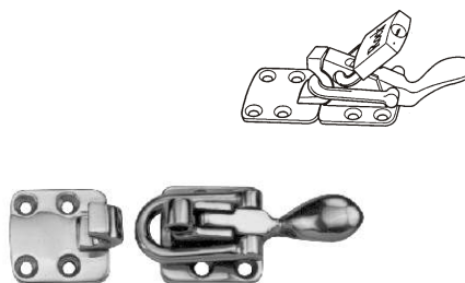
LOCKABLE HOLD DOWN CLAMP casted AISI 316 flat mounting, padlocks not included ITEM NO. Base Screws Weight/g 008303 L3"xW1-1/2"(75x38mm) #8 168
