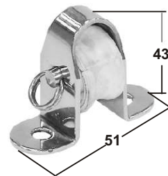
SINGLE LEAD BLOCK AISI 304 For rope \Phi 10 mm plastic sheaves 25x10mm 1sheave pin with split ring can take out. ITEM NO. Weight 012028 35g
