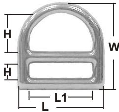
D RING stamped AISI 316
