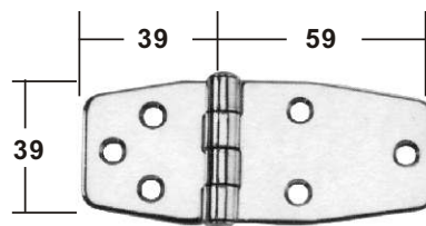
STAMPED AISI 304 buff polished ITEM NO. Thickness Weight/g 006027 2 mm 65 on request AISI 316
