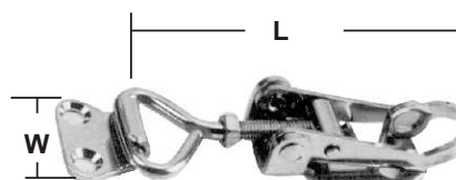
ECCENTRIC LATCH stamped AISI 304 thickness: 1.5mm ITEM NO. adjustable L mm W mm Weight/g 008373 66~75 26 51 008369 115~125 30 116 008368 160~180 35 254
