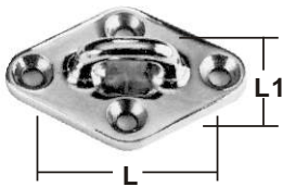
EYE PLATE casted AISI 316
