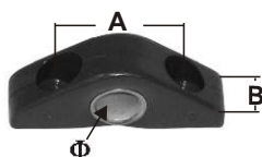
FAIRLEAD Nylon plastic with stainless steel eye ITEM NO. \Phi mm A mm B mm 071600 6 20 14
