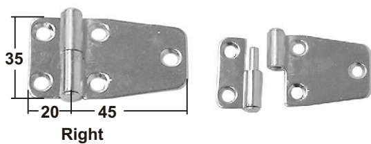
TAKE APART HINGE stamped AISI 304 thickness:2mm ITEM NO. Weight/g 006081 Right 49 006082 Left (no picture) 49 on request AISI 316
