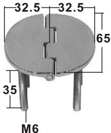
HINGE WITH THREAD precesion casted AISI 316 Reverse ITEM NO. WxL mm Thickness mm Weight/g 008624 65x65(2-9/16"x2-9/16") 4 138
