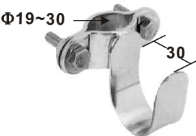
BOAT HOOK HOLDER stamped AISI 304 ITEM NO. Weight/g 007911 132
