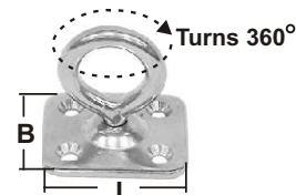
EYE WITH PLATE stamped AISI 304
