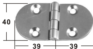
HINGE precision casted AISI 316
