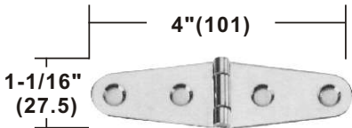
STAMPED AISI 304 buff polished ITEM NO. Thickness Weight/g 006040 1.5 mm 28 on request AISI 316
