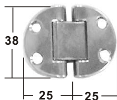
FLUSH 2 PIN HINGE stamped AISI 304 with casted center, buff polished ITEM NO. Thickness Weight/g 006021 1.5mm 30g on request AISI 316
