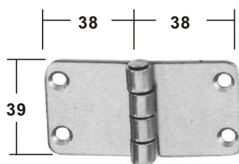
STAMPED AISI 304 buff polished ITEM NO. Thickness Weight/g 006008 2 mm 58 on request AISI 316
