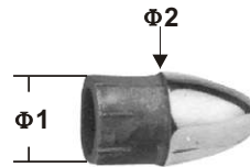
BULLET END PLUG casted AISI 316 ITEM NO. Φ1 mm Φ2 mm Weight 009891 15.5 19 23g 009892 16.5 20 26g 009745 18.5 22 50g 009758 21.5 25.5 50g 009794 26.5 30 50g
