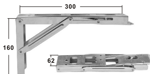
HEAVY DUTY FOLDING BRACKET AISI 304 Folding fitting for tables, and seats made in stainless steel very stable and heavy endure 150kg to the clips for 25mm pipes. ITEM NO. Weight/g 006085 680
