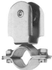
FURLING BLOCK AISI 304 With plastic sheaves to be fitted to a \Phi 25\text{mm} ( \Phi 1" ) stanchion of pulpit ITEM NO. Type Weight 009819 Fixed 105g 009820 Swivel 105g
