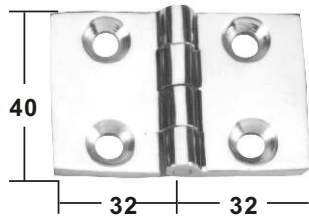
HINGE precision casted AISI 316
