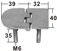
HINGE WITH THREAD precesion casted AISI 316 Reverse ITEM NO. WxL mm Thickness mm Weight/g 008622 40x69(1-9/16"x2-3/4") 4 114
