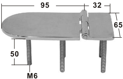
HINGE WITH THREAD precesion casted AISI 316 ITEM NO. WxL mm Thickness mm Weight/g 008620 65x125(2-9/16"x5") 4 320
