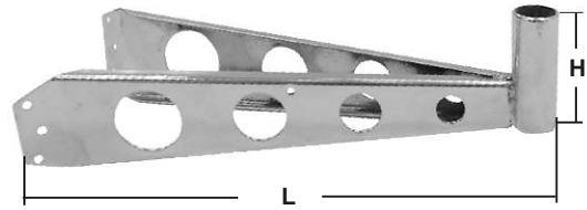
MAST MOUNTING stamped AISI 304 for antenna with 1" 14 thread ITEM NO. L cm H cm 009959 29 7
