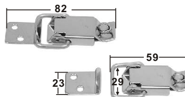
ECCENTRIC LATCH WITH PADLOCK RING stamped AISI 304 ITEM NO. Thickness Weight/g 008360 1.5mm 40
