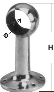
CENTER STANCHIONS casted AISI 316 open ITEM NO. Φ mm H mm Weight 009889 22 87 185g 009762 25 87 165g 009763 40 105 340g
