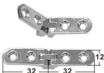
OVAL TABLE HINGES casted AISI 316 hinge locks into place flush with surface when opened. Folds flat at 180° when closed. ITEM NO. Thickness Weight/g 006079 3mm 18
