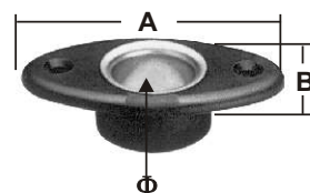
DECK EYE Nylon plastic with stainless steel eye ITEM NO. \Phi mm A mm B mm Weight 071706 6 41 13 4g 071713 13 48 13 10g 071718 18 59 15 16g
