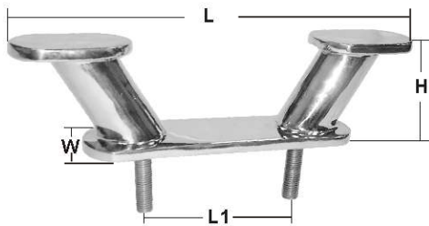
HORN BOLLARD CLEAT casted AISI 316
