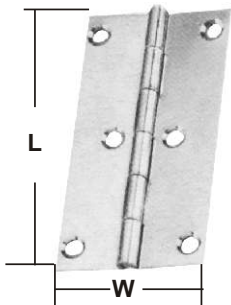
STAMPED AISI 304 buff polished W Thickness L ITEM NO. mm mm mm Weight/g 006125 31 1.5 50 28 006015 54 1.5 100 80 on request AISI 316
