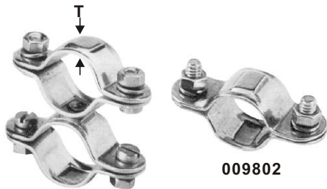
CLAMP stamped AISI 304 ITEM NO. \Phi mm T mm Weight/g 009800 25 1.5 with swivel double 108 009801 25 1.5 double fixed 88 009802 25 1.5 single 43
