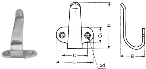
HOOK stamped AISI 304
