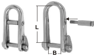
SHACKLE WITH REMOVE PIN
