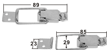
ECCENTRIC LATCH WITH PADLOCK RING stamped AISI 304 ITEM NO. Thickness Weight/g 008361 1.5mm 44
