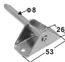
RIGED STERNBRAKET AISI 304 ITEM NO. Weight/g 012039 60
