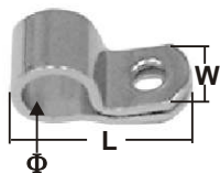
DEAD END BAILS AISI 304 attach any where a dead end is needed for extra purchase. ITEM NO. L mm W mm \Phi mm Weight/g 004316 26 11 9 004317 38 16 13
