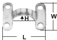
MOUNTING PLATE stamped AISI 304 ITEM NO. L mm W mm H mm Weight/g 004342 42 30 12 9
