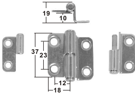
TAKE APART HINGE LEFT stamped AISI 304 ITEM NO. Thickness Weight/g 006064 2mm 40 on request AISI 316
