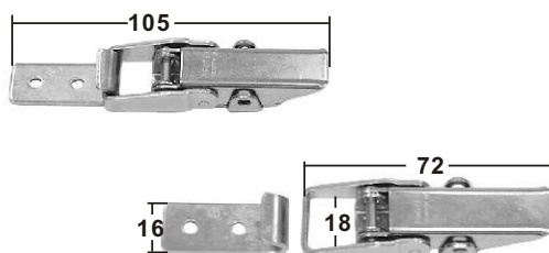
ECCENTRIC LATCH stamped AISI 316 ITEM NO. Thickness Weight/g 008353 1.5mm 50
