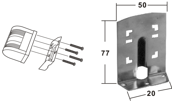
BRACKET FOR LIGHT stamped AISI 304
