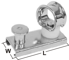
SLIDE WITH ROPE GUIDE stamped AISI 304
