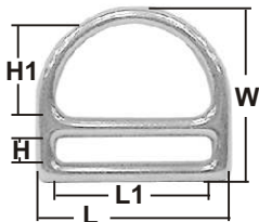
D RING stamped AISI 316
