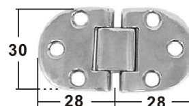
FLUSH 2 PIN HINGE stamped AISI 304 with casted center, buff polished ITEM NO. Thickness Weight/g 006129 1.5mm on request AISI 316
