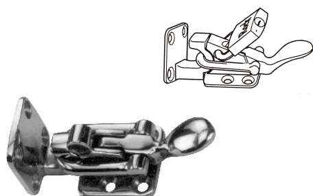
LOCKABLE HOLD DOWN CLAMP casted AISI 316 90° angle mounting, padlocks not included ITEM NO. Base Screws Weight/g 008304 L2-1/2"x1-1/2"(64x38mm) #8 170
