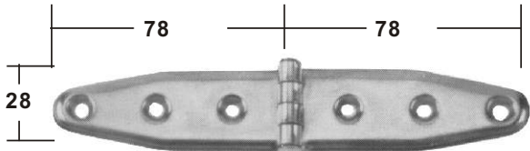
STAMPED AISI 304 buff polished ITEM NO. Thickness Weight/g 006005 1.5 mm 56 on request AISI 316
