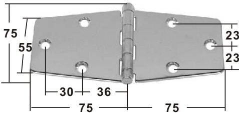
HINGE stamped AISI 304 buff polished ITEM NO. Thickness Weight/g 006074 2 mm 176
