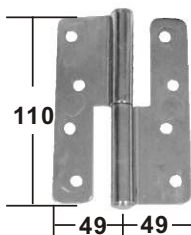
STAINLESS DOOR HINGE stamped AISI 304 buff polished ITEM NO. Size Type Weight/g 007000 110x98mm Left 194 007021 110x98mm Right 194 on request AISI 316
