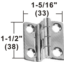
SHORT SIDE OFFSET HINGE stamped AISI 304 buff polished ITEM NO. Thickness Weight/g 006045 1.5 mm 26
