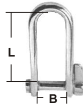
SHACKLE casted AISI 316
