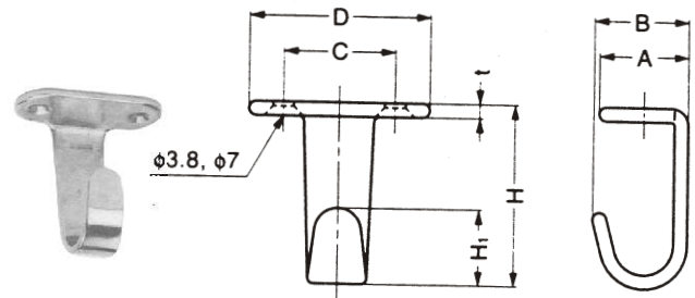
HOOK stamped AISI 304
