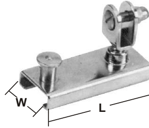
SLIDE WITH STOP END stamped AISI 304 with swivel
