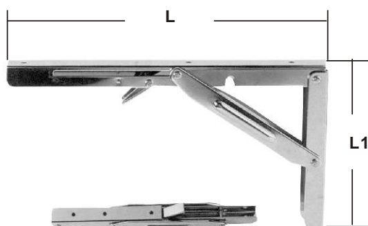
FOLDING BRACKET stamped AISI 304 ITEM NO. L L1 Weight/g 006028 303mm(12") 165mm(6-1/2") 490
