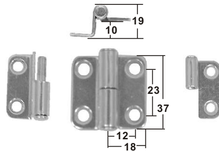
TAKE APART LEFT HINGE RIGHT stamped AISI 304 ITEM NO. Thickness Weight/g 006065 2mm 40 on request AISI 316
