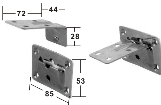
FLUSH MOUNT CONCEALED HINGE stamped AISI 304 ITEM NO. Thickness Weight/g 006019 2mm 258
