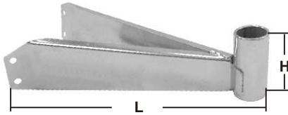
MAST MOUNTING stamped AISI 304 for antenna with 1" 14 thread ITEM NO. L cm H cm 009958 19 7
