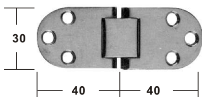
FLUSH 2 PIN HINGE stamped AISI 304 with casted center, buff polished ITEM NO. Thickness Weight/g 006022 1.5mm 43 on request AISI 316
