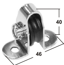
SINGLE LEAD BLOCK AISI 304 For rope \Phi 6 mm plastic sheaves 25x9.2mm 1sheave pin with split ring can take out. ITEM NO. Weight 012027 31g
