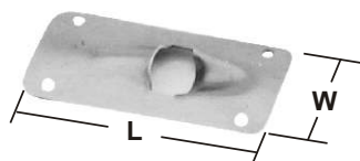
HALYARD EXIT PLATES AISI 304 stamped ITEM NO. LmmxWmm Type Weight/g 003707 88x32(3-1/2"x1-1/4") curved 30 003708 88x32(3-1/2"x1-1/4") flat 30 003709 117x51(4-5/8"x2") flat 120 003715 117x51(4-5/8"x2") curved 120
