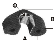
FAIRLEAD Nylon plastic with stainless steel eye ITEM NO. \Phi mm A mm B mm 071601 6 23 15 071602 8.5 25 20
