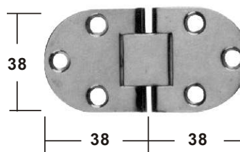
FLUSH 2 PIN HINGE stamped AISI 304 with casted center, buff polished ITEM NO. Thickness Weight/g 006023 1.5mm 45 on request AISI 316
