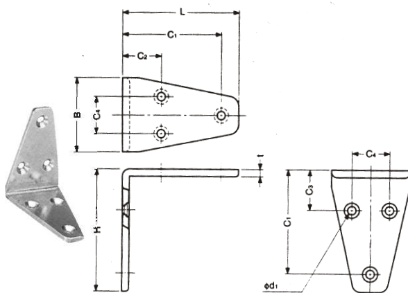
ANGLES stamped AISI 304
