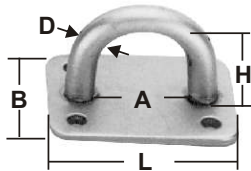
EYE PLATE stamped AISI 304
