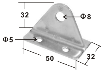
SHROUD PLATE stamped AISI 304 ITEM NO. Weight/g 004301 37 on request AISI 316
