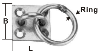
ROUND RING WITH PLATE stamped AISI 304
