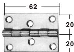
STAMPED AISI 304 buff polished ITEM NO. Thickness Weight/g 006007 1.5 mm 39 on request AISI 316
