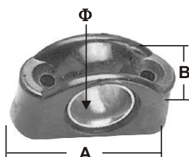
DECK EYE Nylon plastic with stainless steel eye ITEM NO. \Phi mm A mm B mm Weight 071606 6 36 22 3g 071613 13 41 23 4g 071617 17 55 31 36g
