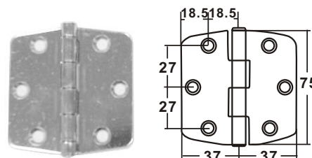
FLUSH DOOR HING stamped AISI 304 buff polished ITEM NO. Thickness Type Weight/g 006004 2 mm 105 006088 2 mm reverse 105 on request AISI 316
