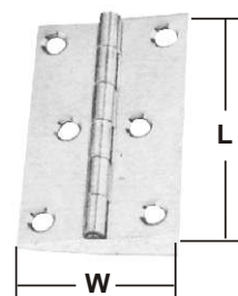
BUTT HINGE stamped AISI 304 thickness:2mm buff polished ITEM NO. L mm W mm Weight/g 006013 77x50 (3"x2") 56 006025 77x77 (3"x3") 80 on request AISI 316
