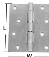
HING stamped AISI 304 ITEM NO. L mm W mm Thickness Weight/g 008829 80(3-1/8") 100(4") 2 mm 164 008837 100(4") 100(4") 3 mm 294 008843 120(4-3/4") 100(4") 3 mm 354 on request AISI 316
