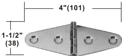
STAMPED AISI 304 buff polished ITEM NO. Thickness Weight/g 006041 1.5 mm 36 on request AISI 316
