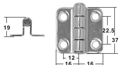
HINGE stamped AISI 304 ITEM NO. Thickness Weight/g 006066 2mm 46 on request AISI 316
