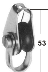
BLOCK AISI 304 For rope \Phi 10 mm plastic sheaves 20x10mm sheaves with becket ITEM NO. Weight 016120
